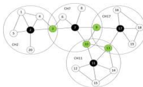
Figure 4: Clustering Architecture
