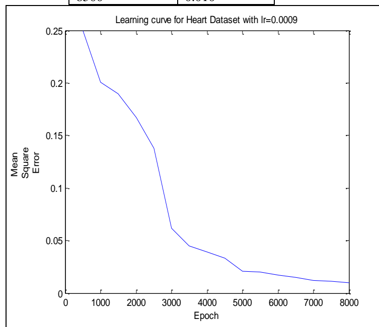
Figure 1 Learning curve for Heart dataset with lr=0.0009
