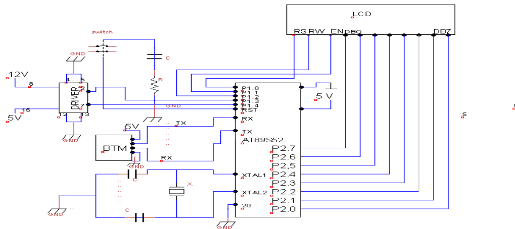
Fig. 4 Schematic Diagram of the Complete System
