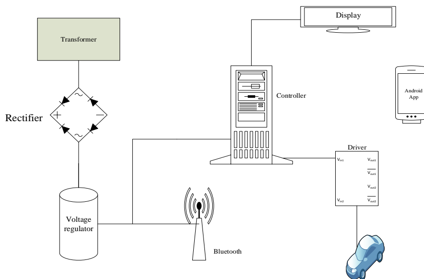
Fig.2 Instrument Setup
