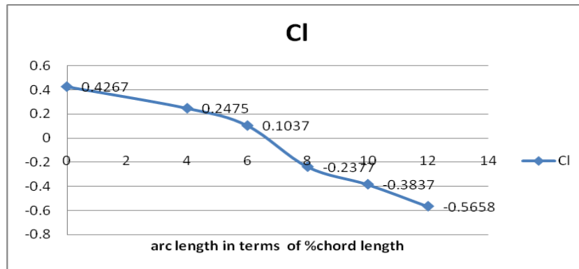
Figure 9. Arc length as % of chord length vs lift coefficient
