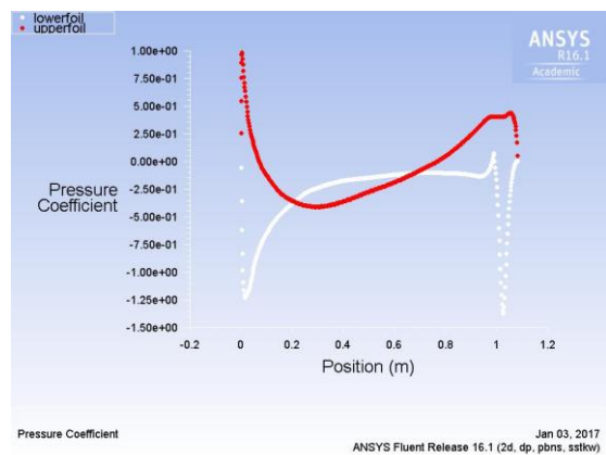
Figure 14. Cp with reflected arc length 8% C
