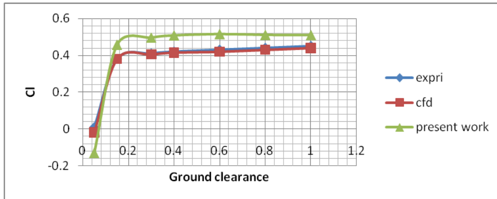
Figure 5 Coefficient of Lift at different height at 0° AOA
