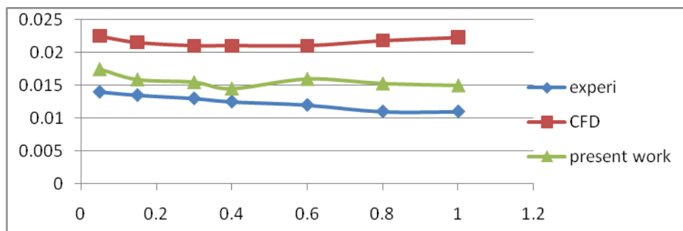
Figure 8 Coefficient of Drag at different height at 6° AOA
