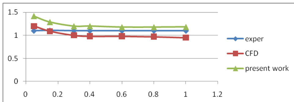
Figure 7 Coefficient of Lift at different height at 6° AOA
