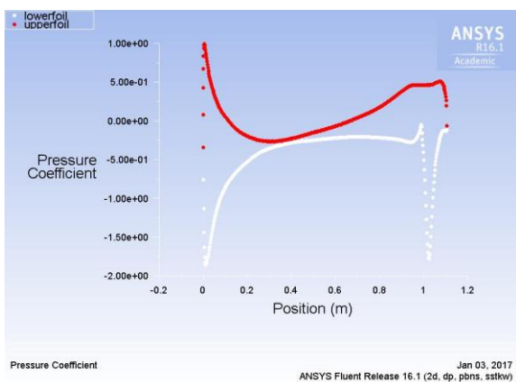
Figure 16. Cp with reflected arc length 12% C
