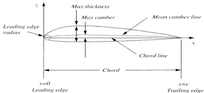
Figure 1 nomenclature of airfoil
