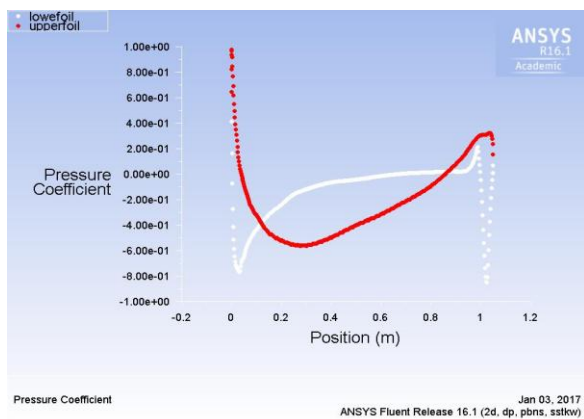
Figure 13. Cp with reflected arc length 6% C
