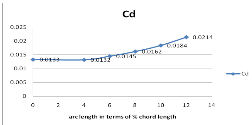
Figure 10. Arc length as % of chord length vs drag coefficient
