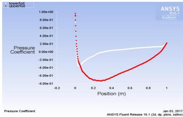
Figure 11. Cp of naca4412
