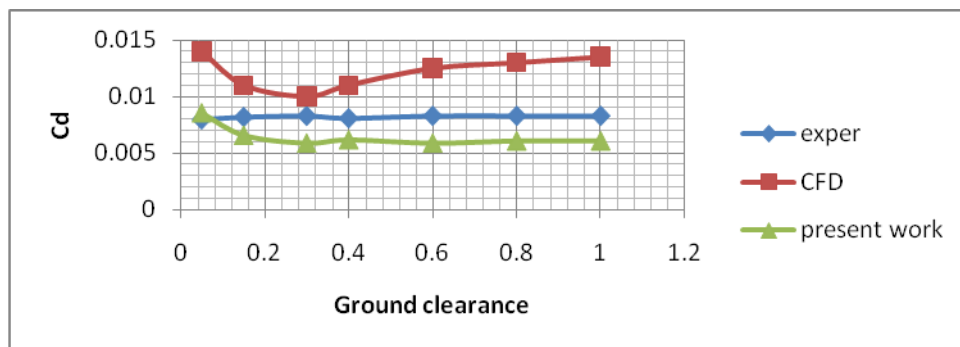
Figure 6 Coefficient of Drag at different height at 0° AOA
