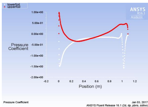
Figure 15. Cp with reflected arc length 10% C
