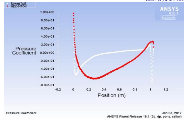
Figure 12. Cp with reflected arc length 4% C
