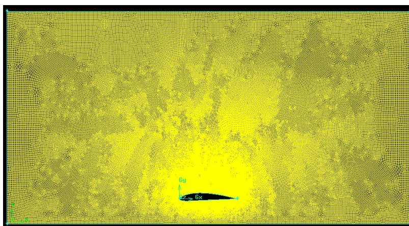
Figure 4 Close up of grid around NACA4412 at 0^{\circ} AOA at H/C 0.4
