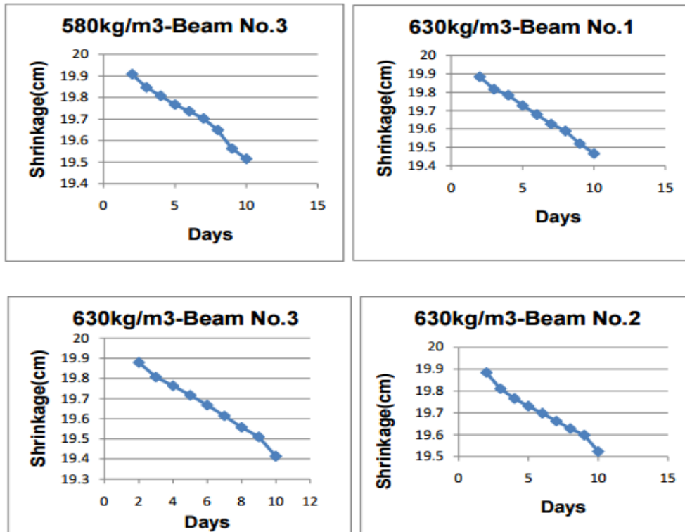
Fig.8 Graphical representation of shrinkage loss before releasing of pre-stressed force (1200x120x120)mm
