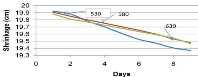
Fig.10.Shrinkage comparison of different powder content
