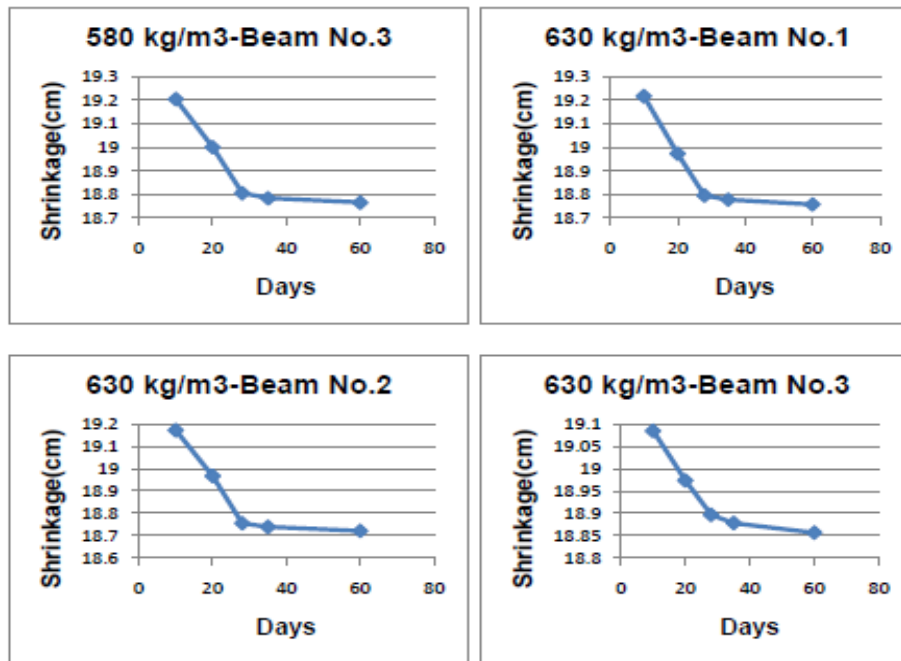
Fig.9 Graphical representation of shrinkage loss after releasing of prestressed force (1200x120x120)mm
