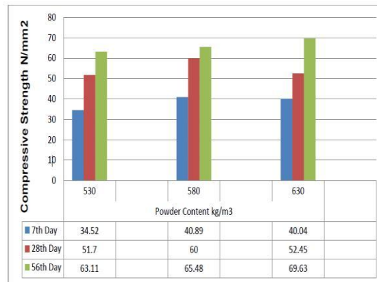
Fig.7 Graphical comparison for compressive strength
