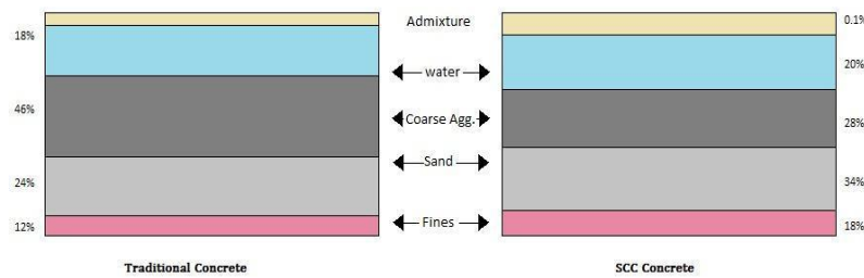
Fig.2 Comparison between traditional concrete & SCC
