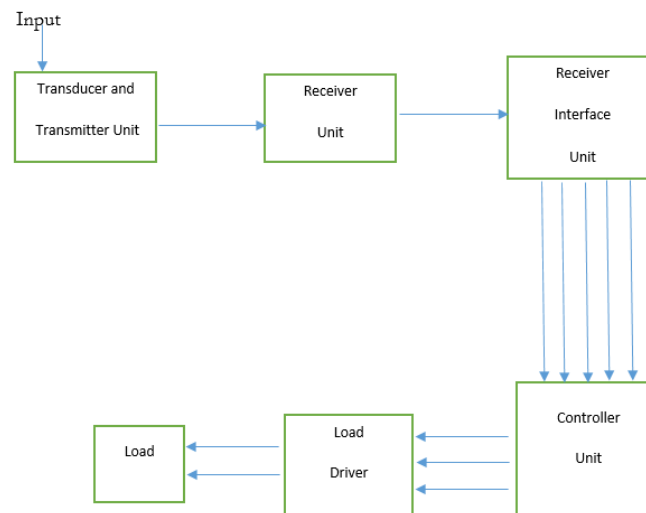
Fig. 1 Functional Block Diagram of Gesture Controlled Home Automation
