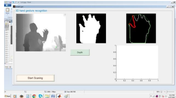
Fig. 3. Polygonal Approximation
