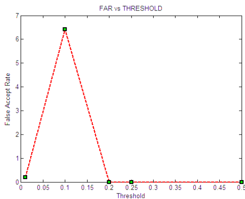
Fig3. GCF FAR against Threshold.
