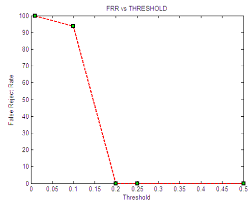
Fig4. GCF FRR against Threshold.
