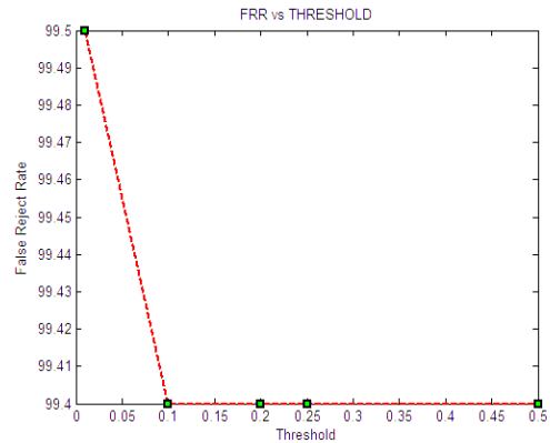
Fig.10 Y-axis on Bottom FRR against Threshold.
