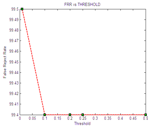
Fig7. X-axis on RH FRR against Threshold.
