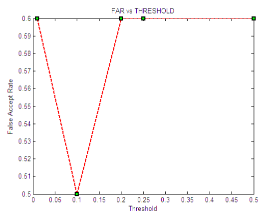
Fig6. X-axis on RH FAR against Threshold.
