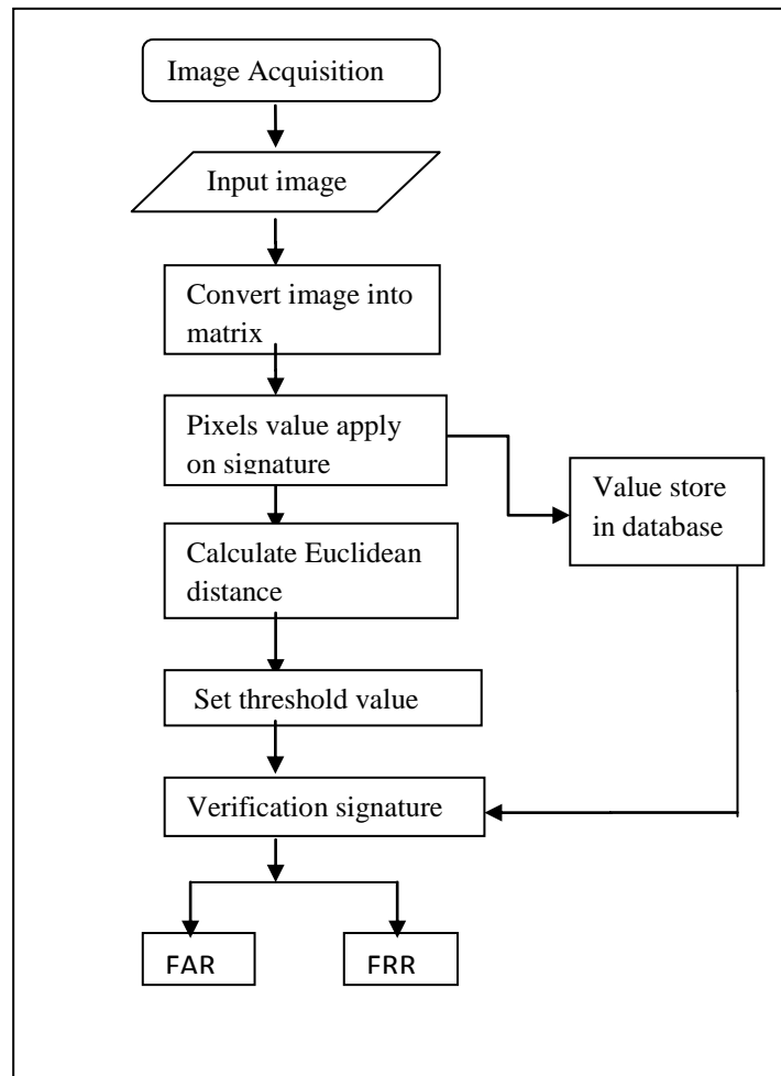
Fig.2 Flowchart of signature identification.
