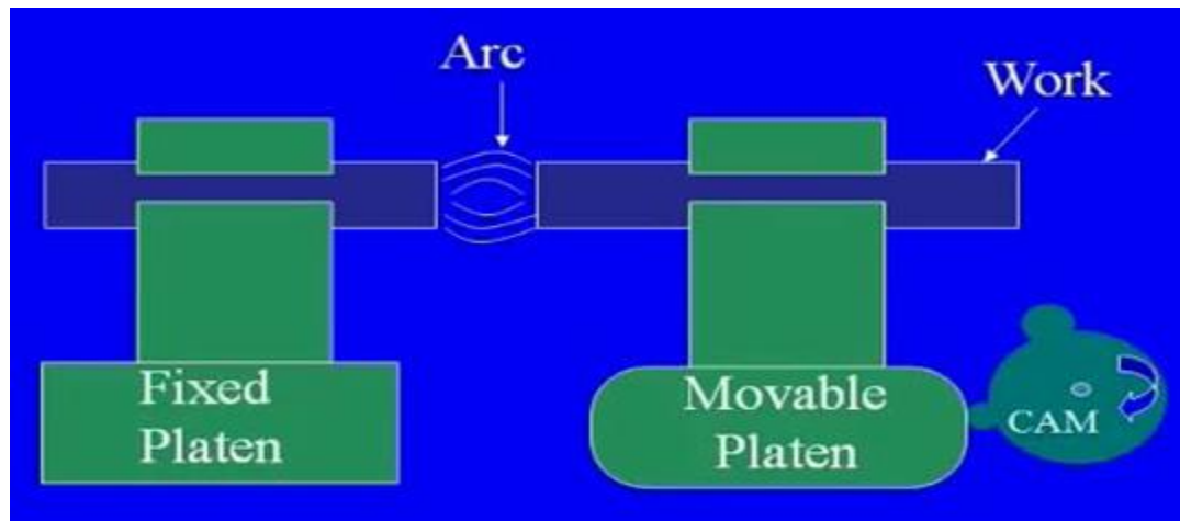
Figure: Schematic of Flash Welding
