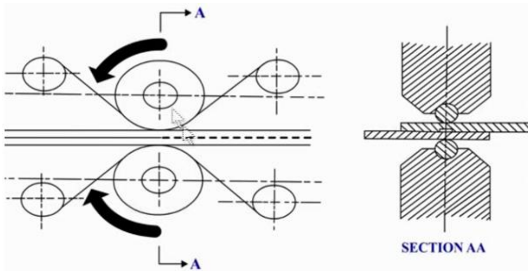
Figure: Schematic of the Electrode Wire Seam Welding Process
