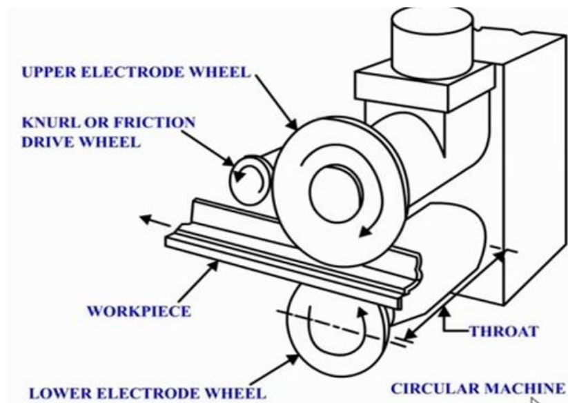
Figure: Schematic of the resistance seam welding process
