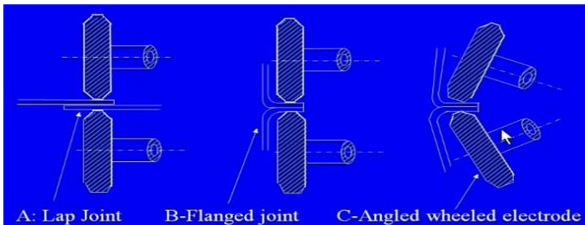
Figure: Types of Projection Welding
