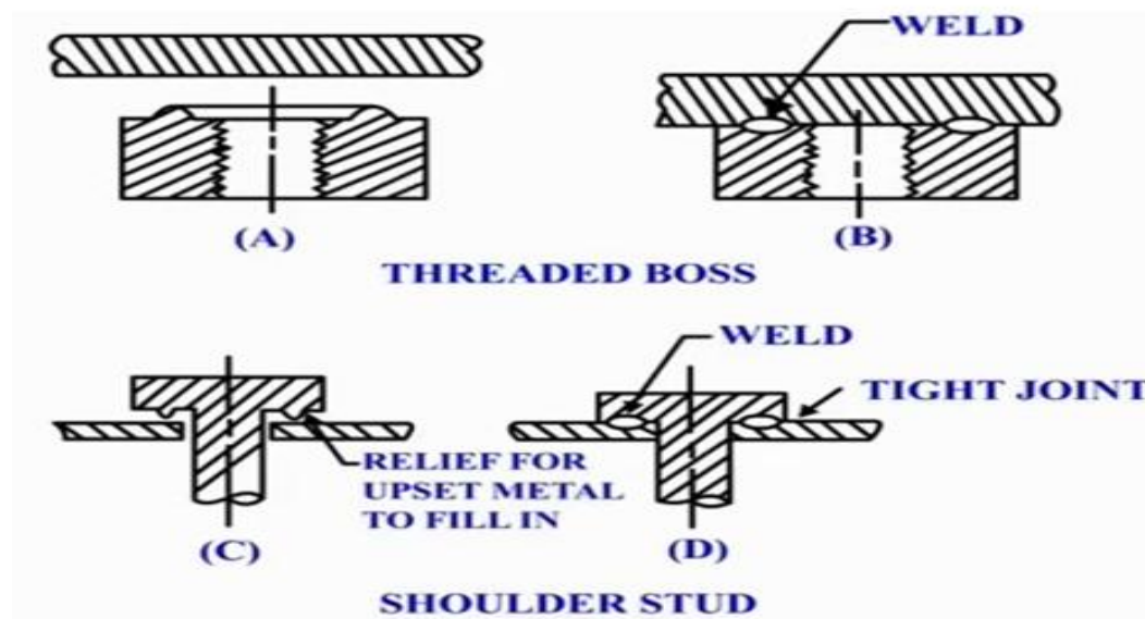
Figure: Projection Welding Design
