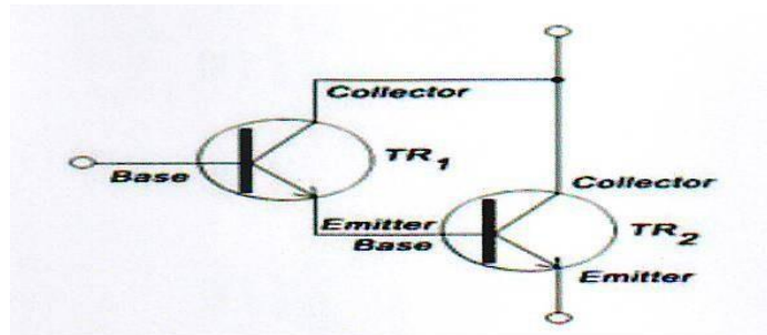
Fig. 8: Darlington Pair
