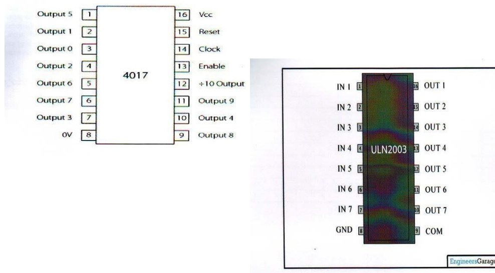
Fig.7: Pin configuration
