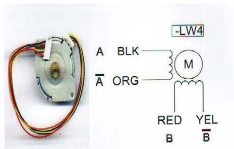
Fig. 8: Stepper motor & its internal diagram
