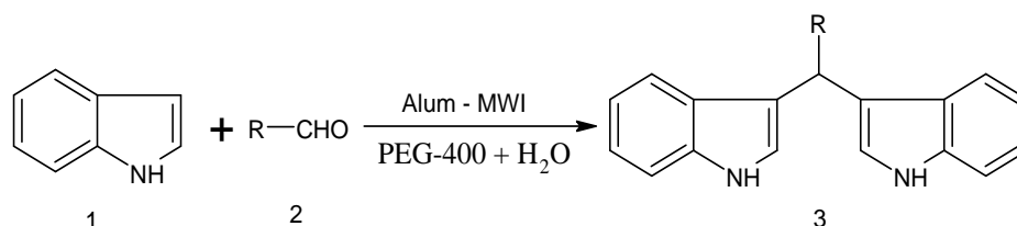
Scheme I: Synthesis of bis-(indolyl)methanes in Polyethylene Glycol and Water as green media Using Microwave Irradiation.
