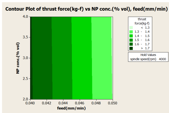
Fig 9 Feed rate vs volume concentration
