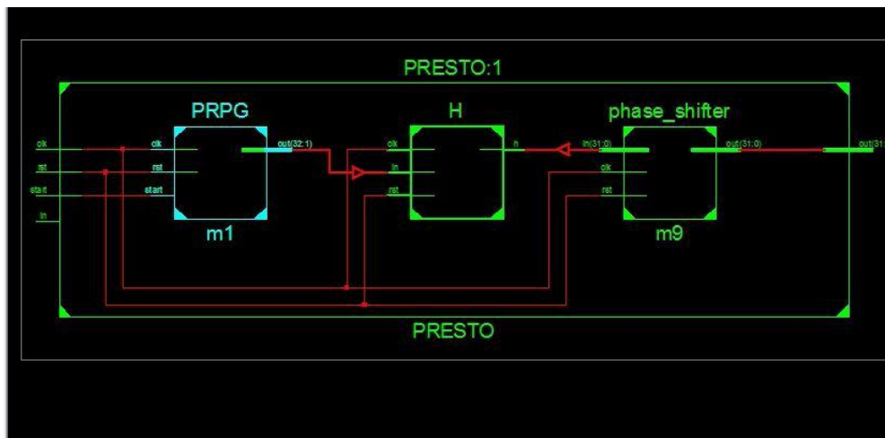
Fig.5 Presto Schematic
