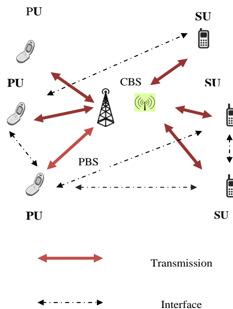
Fig.1 System model of OFDM based cognitive radio system
