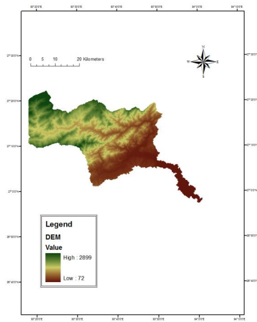
Figure 3: Dikrong DEM
