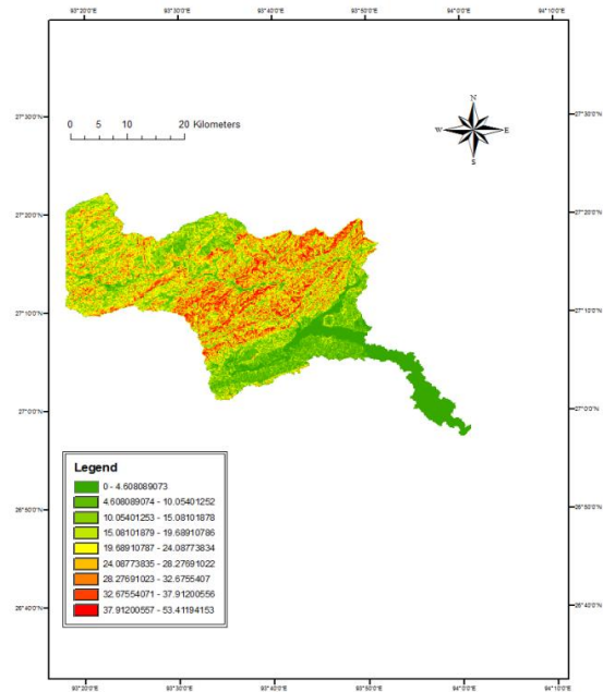
Figure 5: Slope map of Dikrong
