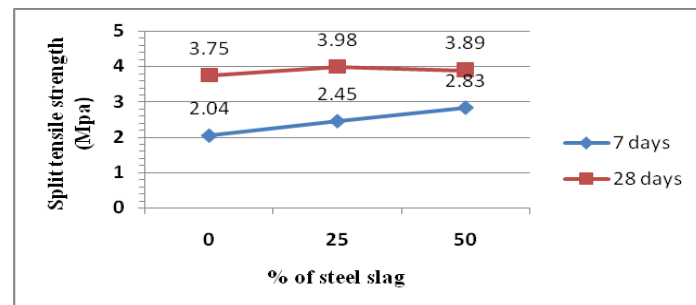
Fig 5 Split tensile strength of concrete
