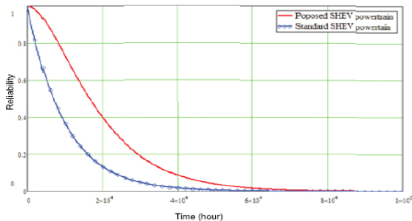
Fig. 4. Reliability functions of the proposed and standard SHEV powertrains.
