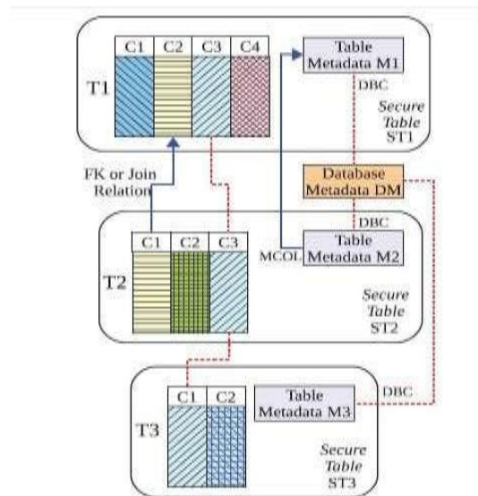
Fig. 4. Management of the encryption keys according to the field confidentiality parameter.
