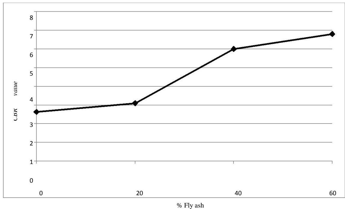
Fig.6. CBR value variations for stabilized soil.
