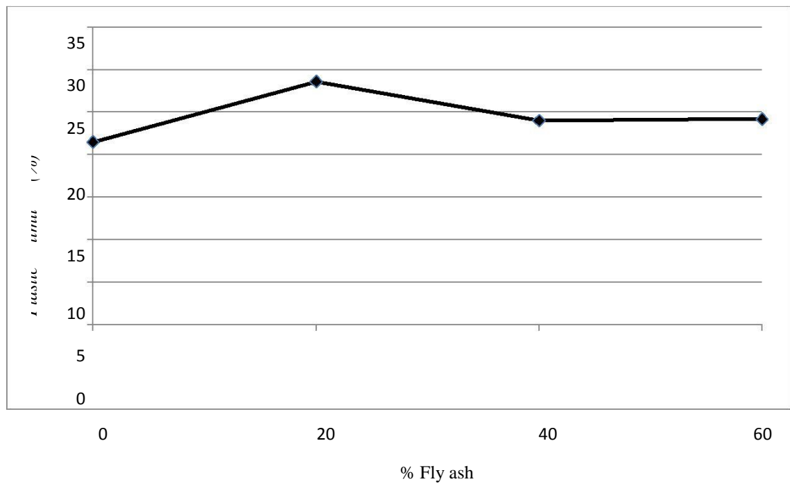
Fig.2. Plastic limit variations for stabilized soil.
