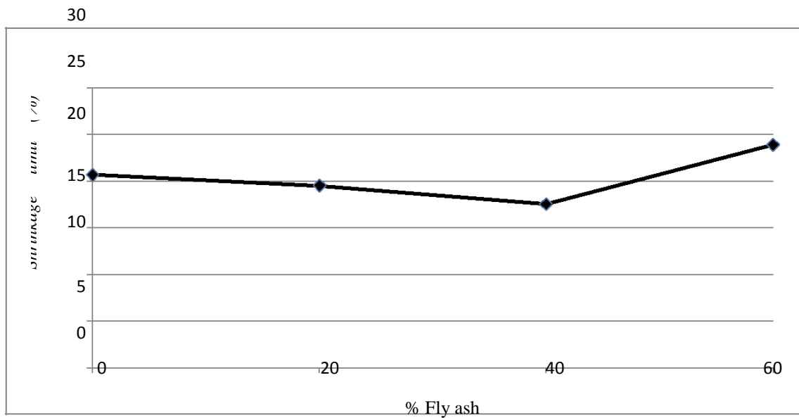
Fig.3. Shrinkage limit variations for stabilized soil.
