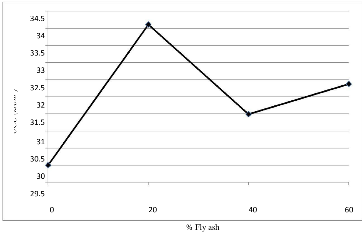
Fig.5.Strength variations for stabilized soil.
