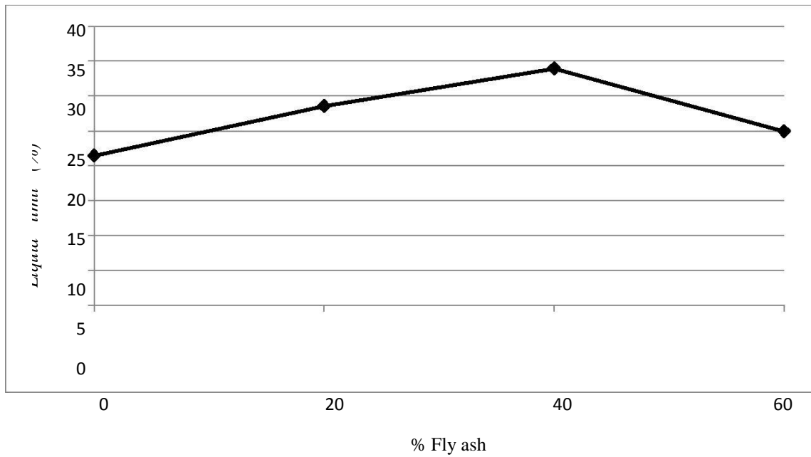
Fig.1. Liquid limit variations for stabilized soil.
