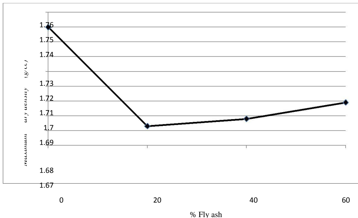
Fig.4. Maximum dry density variations for stabilized soil.
