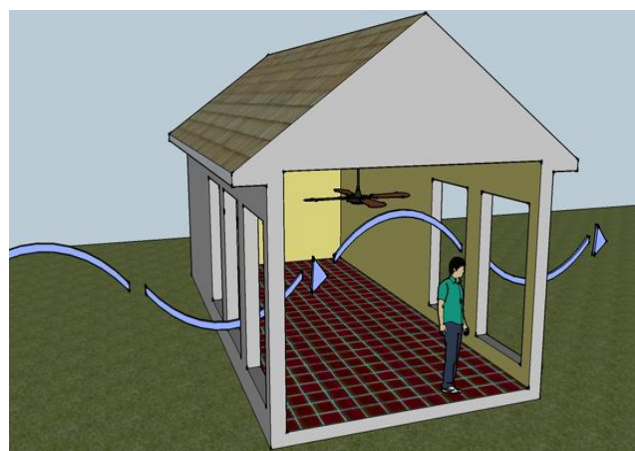
Fig.2.1cross ventilation
