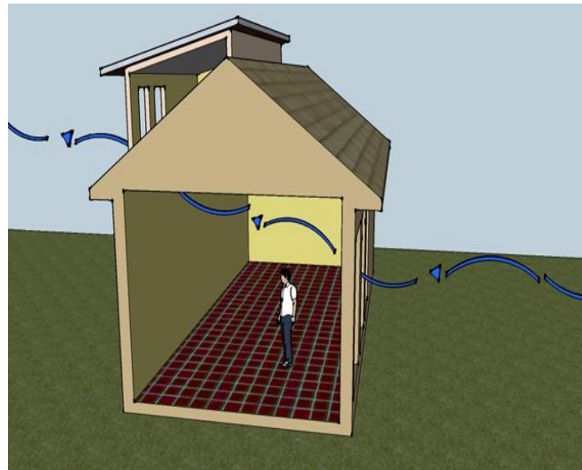
Fig.2.2 stack ventilation
