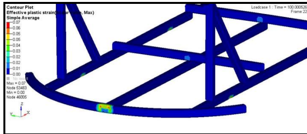
PLASTIC STRAIN ANALYSIS OF STRUCTURE
