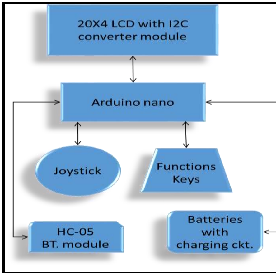
Fig.2.Block Diagram Of Remote Control
