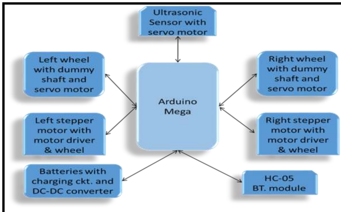
Fig . 1. Block Diagram Of Convertible Self Blancing Robot
