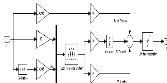
Figure 3. Simulation of Fuzzy PID Controller
