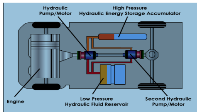
Figure 4: Series Hydraulic Hybrid Drive
