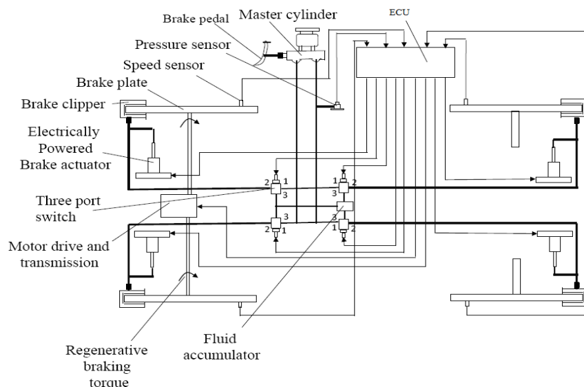
Figure 6: Line diagram of electronically controlled regenerative braking system acts as ABS.
