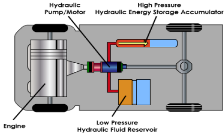
Figure 2: Parallel Hydraulic Hybrid Drive
