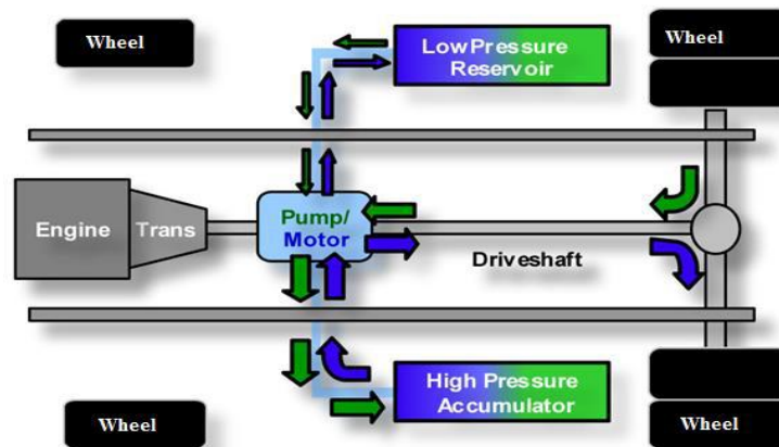
Figure 3: Hydraulic Launch Assist (HLA) System
