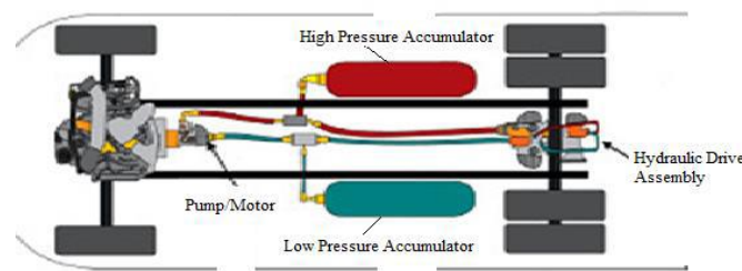
Figure 5: UPS Truck with Series Hydraulic Hybrid drive
