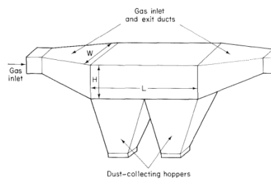
Fig. 1 Settling Chamber
