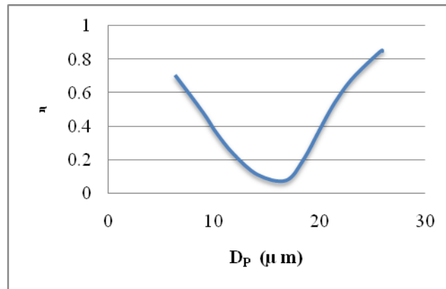
Fig. 7 Overall efficiency of the electrostatic precipitator
