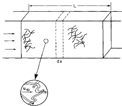
Fig. 4 Filter bed composed of an assemblage of single fibers
