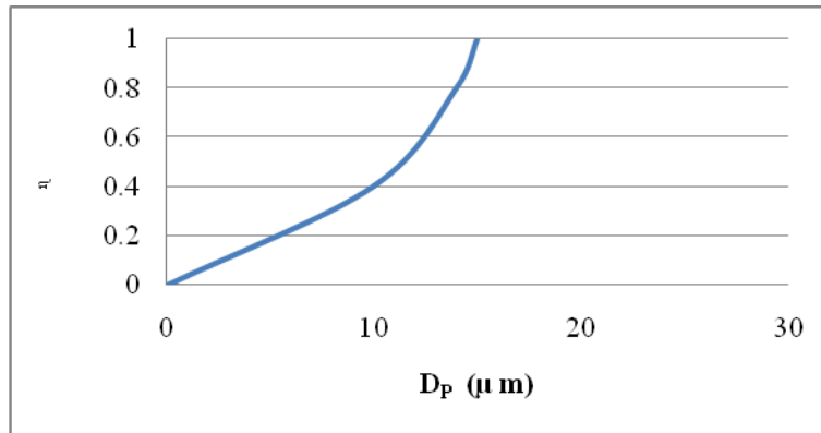
Fig. 5 Cyclone efficiency of laminar flow particle as the particle size increases the efficiency also increases so it can be said that efficiency is a function of particle size
