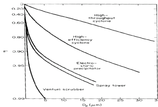
Fig. 8 Comparison of efficiencies
