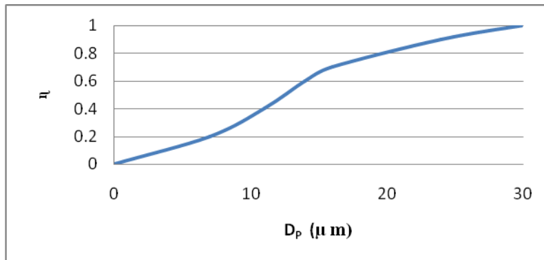
Fig.6 Cyclone efficiency of turbulent flow particle
