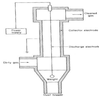
Fig.3Cylindrical single-stage electrostatic precipitator
