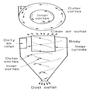
Fig. 2 Tangential inlet vertical reverse flow cyclone
