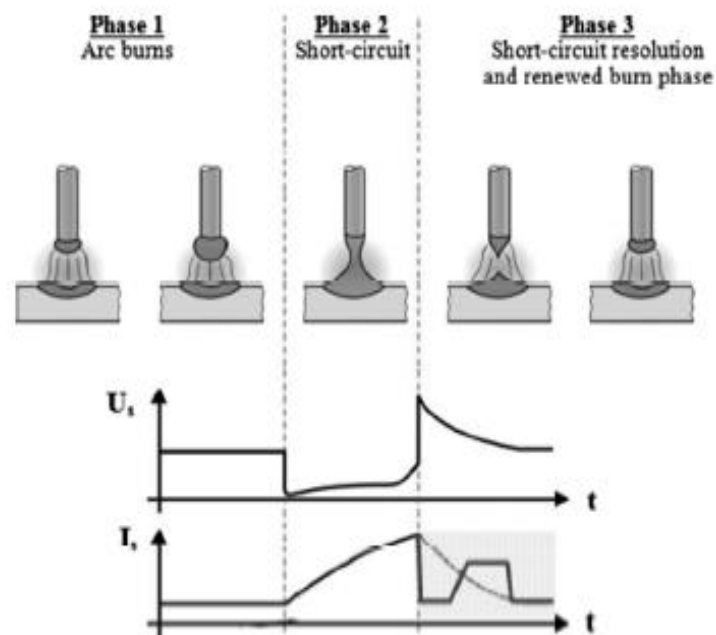
Fig. 2. Principle of cold arc technology, replotted from [1].
