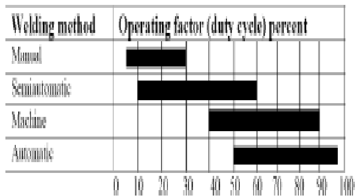
Fig. 1. Effect of mechanization on operator factor, reported from [6].
