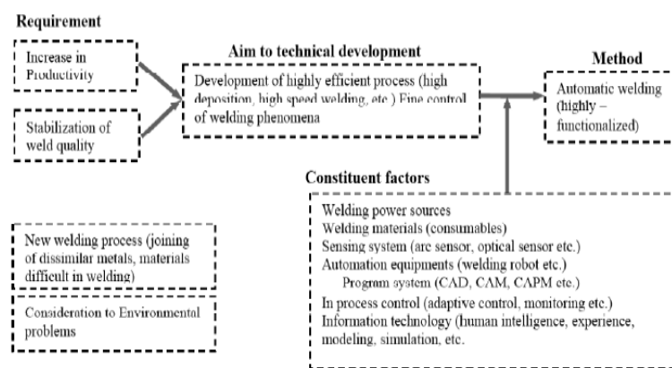
Fig.3. Requirements for welding production technology permitting its integration to automatization.
