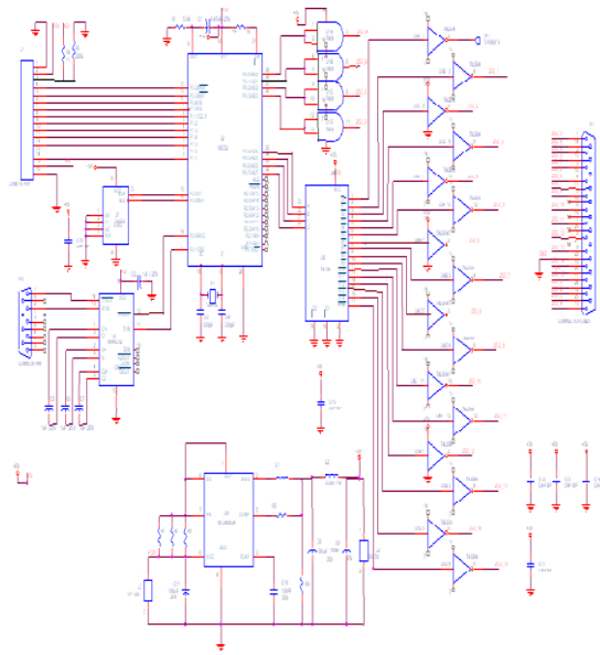
Fig 3: circuit diagram of receiver section.
