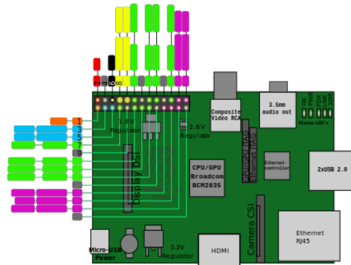
Fig 6: Pinout-diagram for Rev. 1 Board
