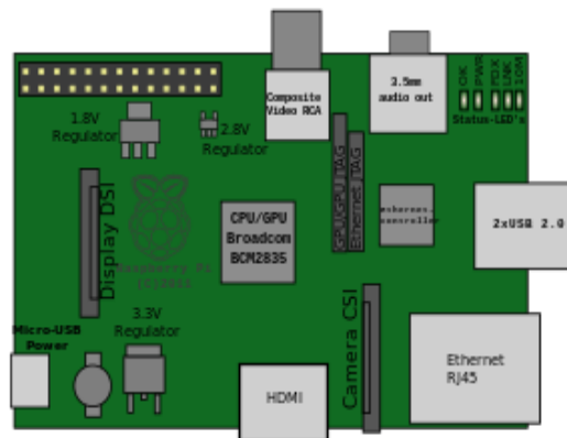
Fig 5: Location on the PCB of connectors and major ICs
