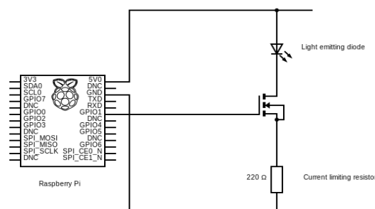
Fig 7: Using GPIO pins to control an LED
