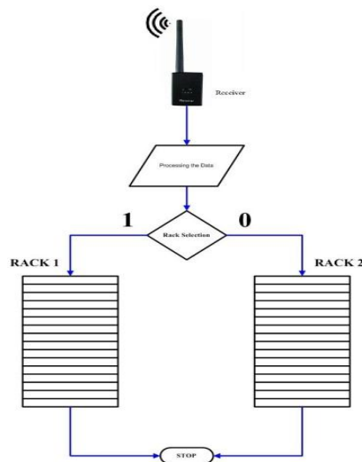
Fig 4: flow chart for hardware realization
