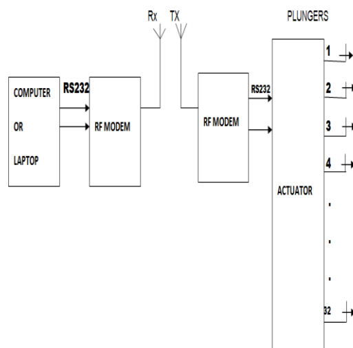
Fig 1 block diagram of the project
