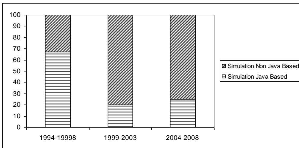
Figure 4: Simulation Packages
