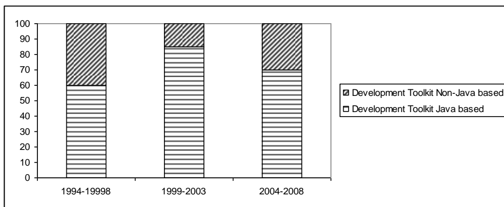
Figure 1: Development Toolkit
