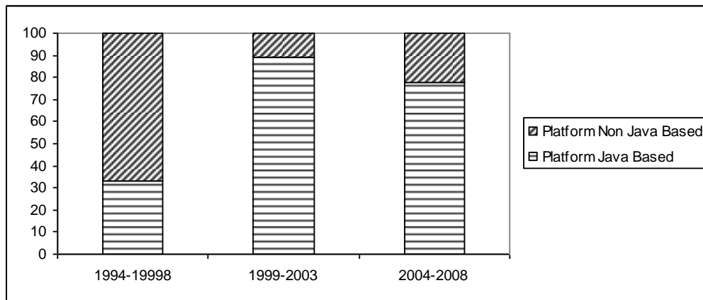
Figure 3: Platforms
