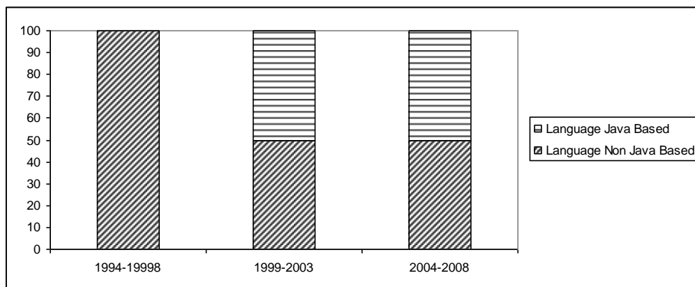
Figure 2: Languages
