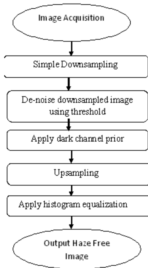
Figure 2 Purposed Dehazing Algorithm
