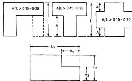
Figure 2.1 Re-entrant Corners plan irregularity
