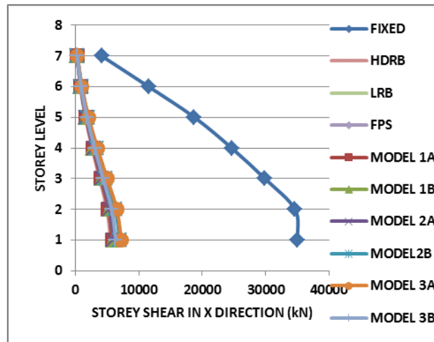
Figure 4.5 Storey shear in x-direction
