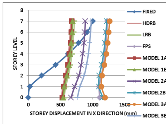
Figure 4.6 Storey Displacement in x-direction
