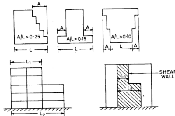
Figure 2.2 Vertical Geometric Irregularity
