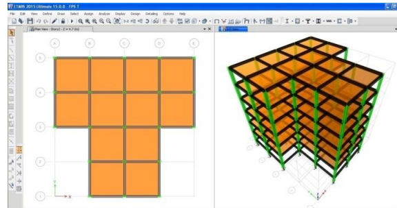
Figure 3.1. T shape plan irregular building
