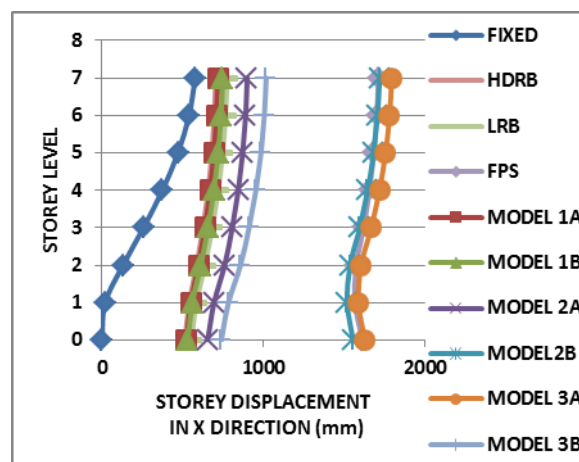
Figure 4.3 Storey Displacement in x-direction
