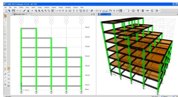
Figure 3.2. Vertical geometric irregular building
