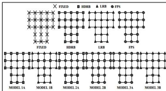
Figure 3.3 Plan irregular building plan
