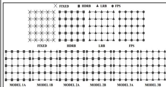
Figure 3.4 Vertical irregular building plan
