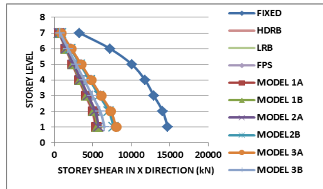
Figure 4.2 Storey shear in x-direction
