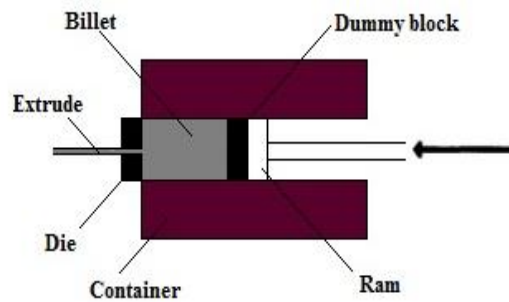
Figure 1: Schematic of Direct Extrusion Process
