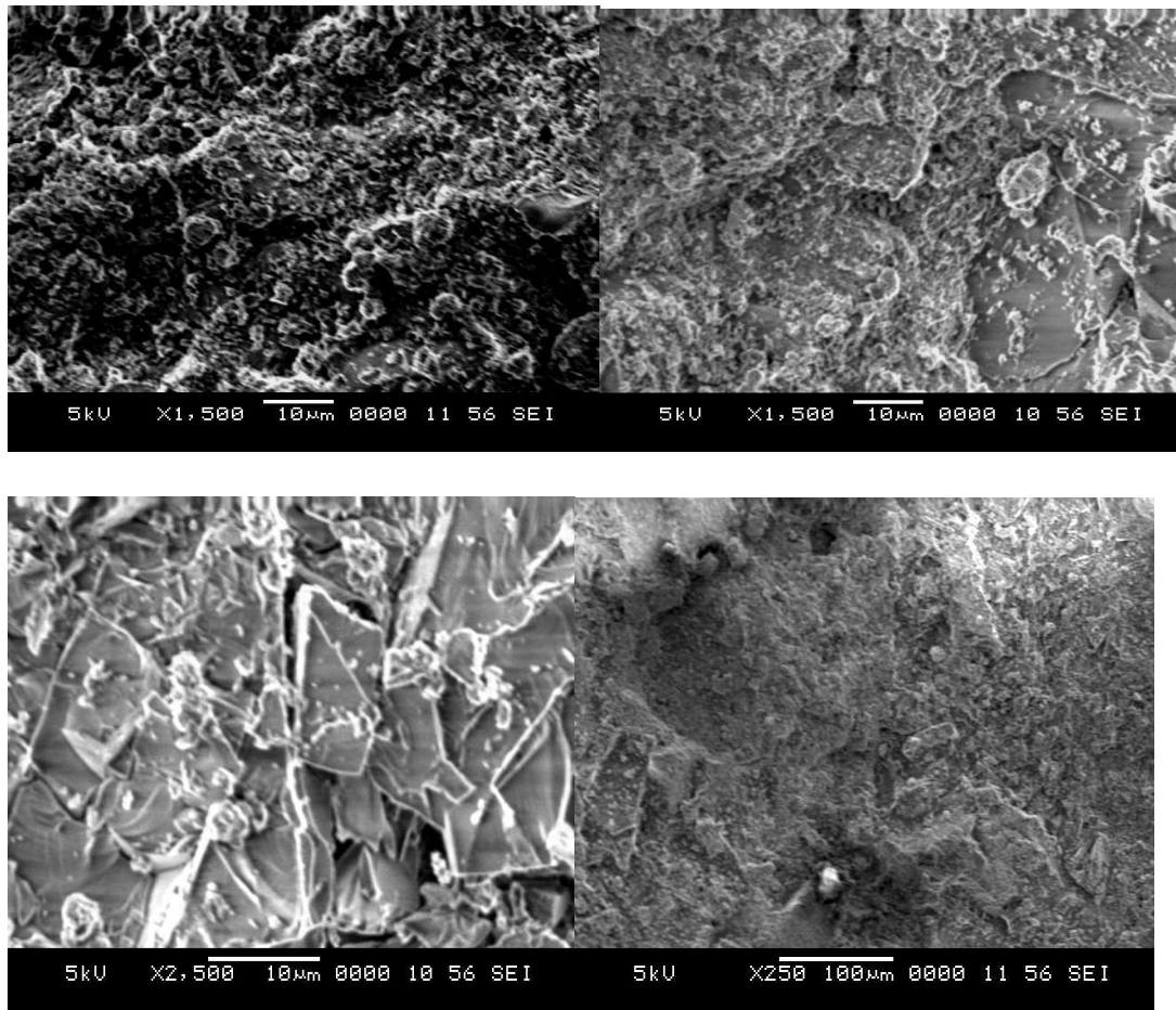
Fig. 6: SEM images of M 100 0% RHA
