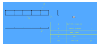
Assembly
