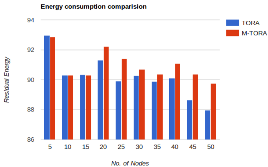
Figure 2: Energy consumption comparison
