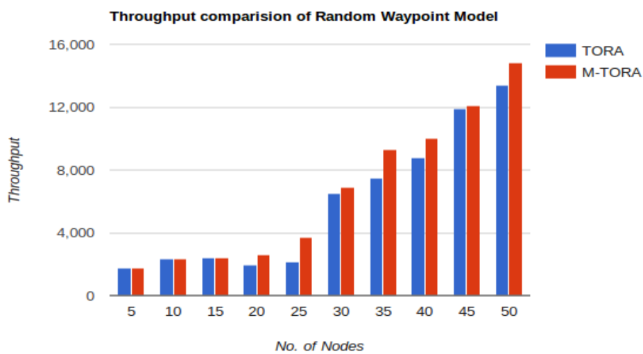
Figure 3: Throughput Comparison in Random Waypoint Model
