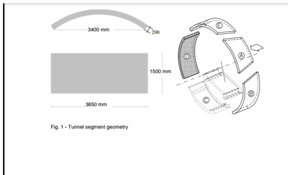
Fig.1 Tunnel segment geometry
