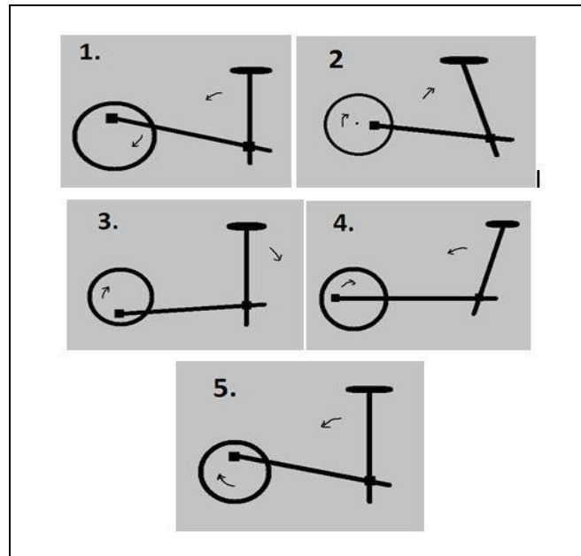
Fig 2: Different Position of Single Slider Mechanism
