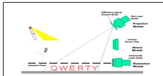
Fig 2: Physical setup of system [4]
