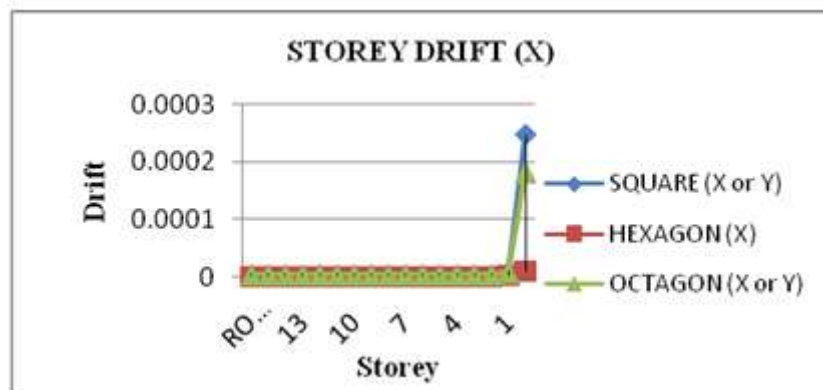
Fig.5.7 Storey Drift (X)
