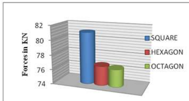
Fig.5.6 Column Axial Forces
