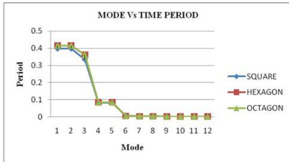
Fig.5.11 Mode Vs Time Period
