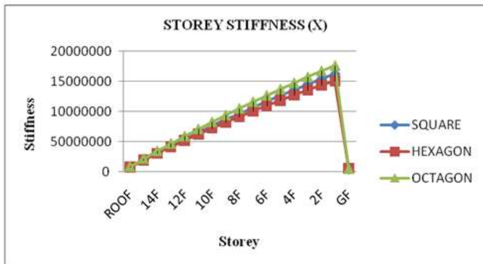
Fig.5.9 Storey Stiffness (X)
